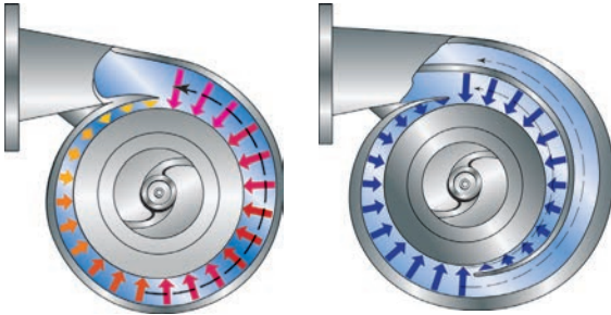
Single Volute
